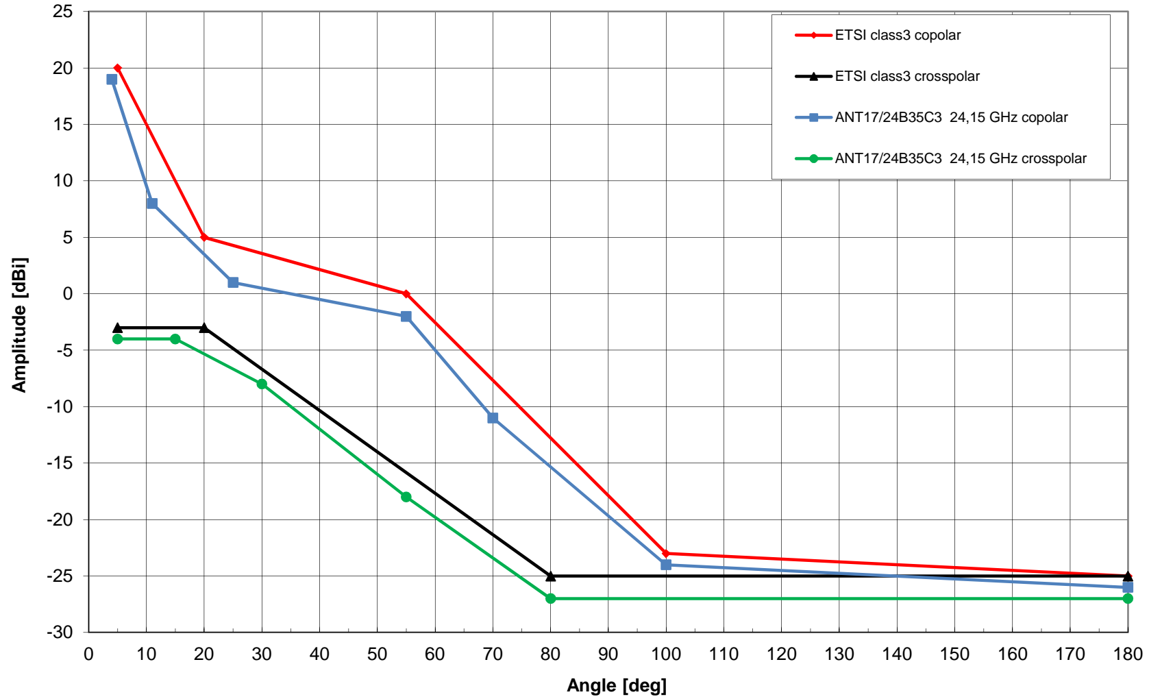
Radiation pattern ANT17/24B35C3 24,15 GHz, max. gain 36,0 dBi
