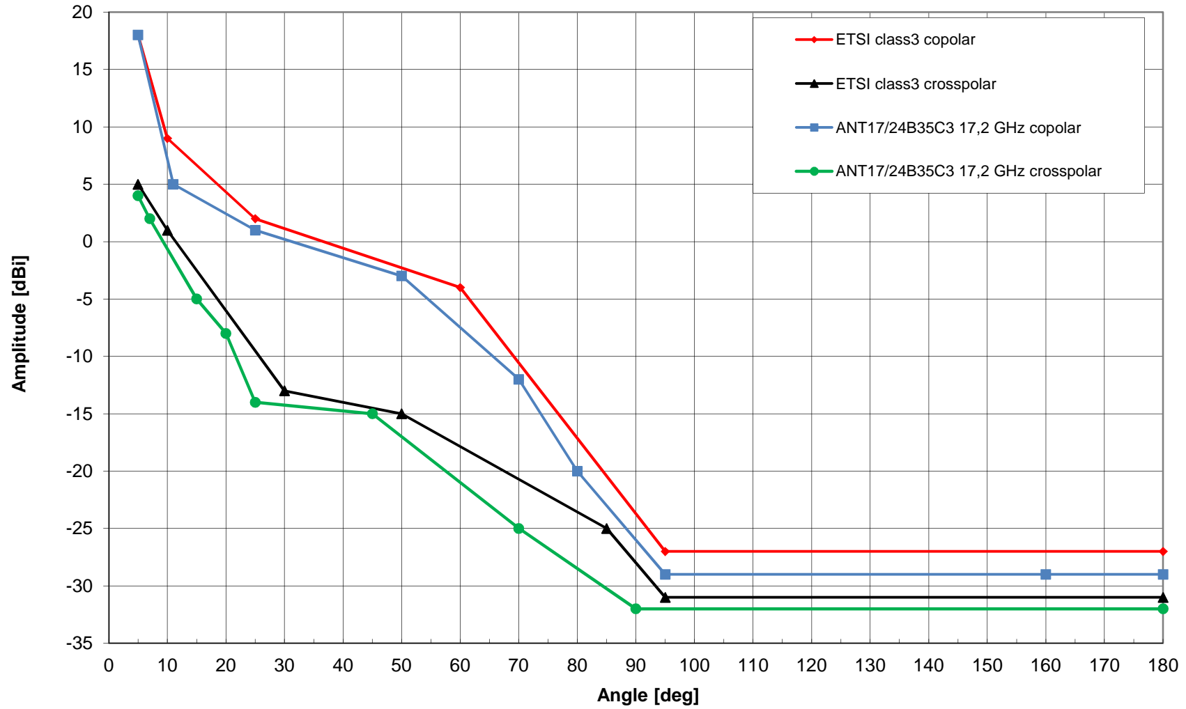
Radiation pattern ANT17/24B35C3 17,2 GHz, max. gain 33,0 dBi
