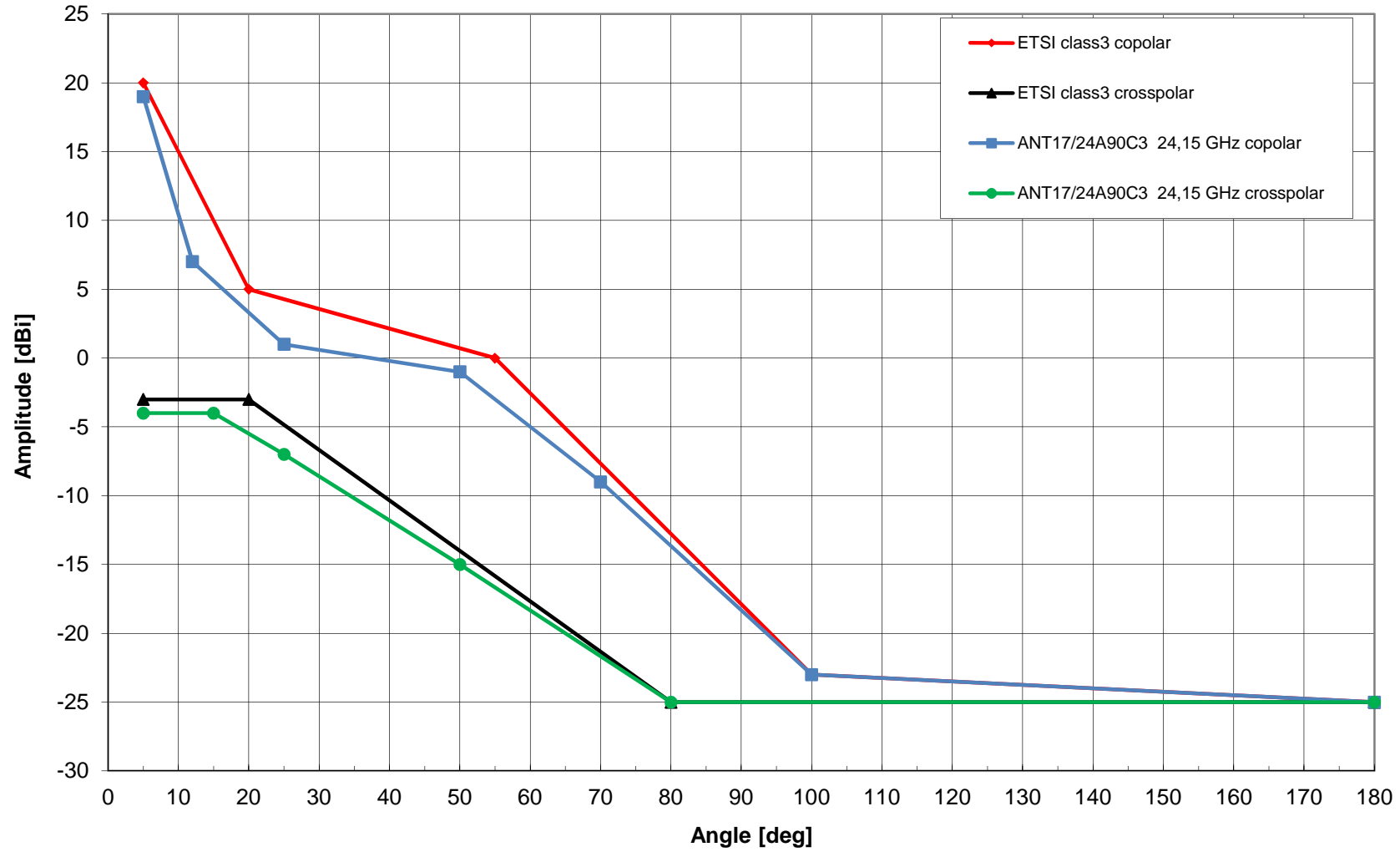
Radiation pattern ANT17/24A90C3 24,15 GHz, max. gain 44,0 dBi
