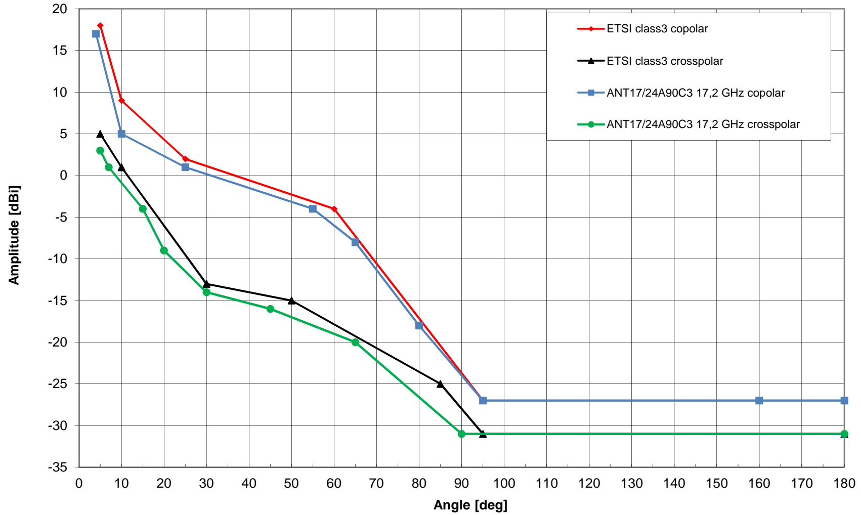
Radiation pattern ANT17/24A90C3 17,2 GHz, max. gain 41,0 dBi
